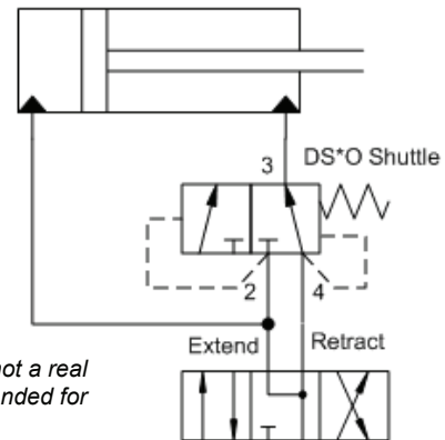
Figure 4. Full Time Regeneration with Cylinder Float in Neutral
