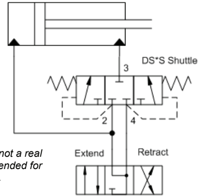
Figure 3. Full Time Regeneration with Rod End Blocked in Neutral
