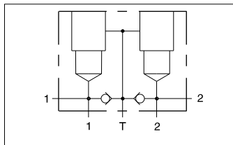
Two cavity body with make-up checks for cross-port relief applications.
